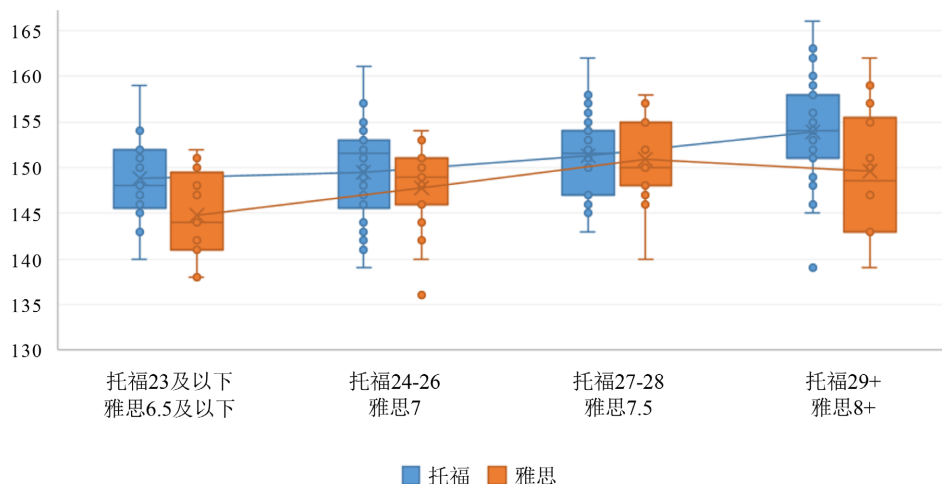
Figure 2. Boxplot of students' GRE verbal scores under the same TOEFL/IELTS reading level 图 2. 托福/雅思阅读对标分数下学员 GRE 语文成绩箱线图
