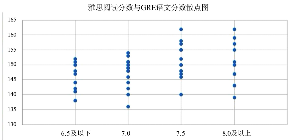
Figure 3. Scatter plot of IELTS reading scores and GRE verbal scores 图 3. 雅思阅读分数与 GRE 语文分数散点图
