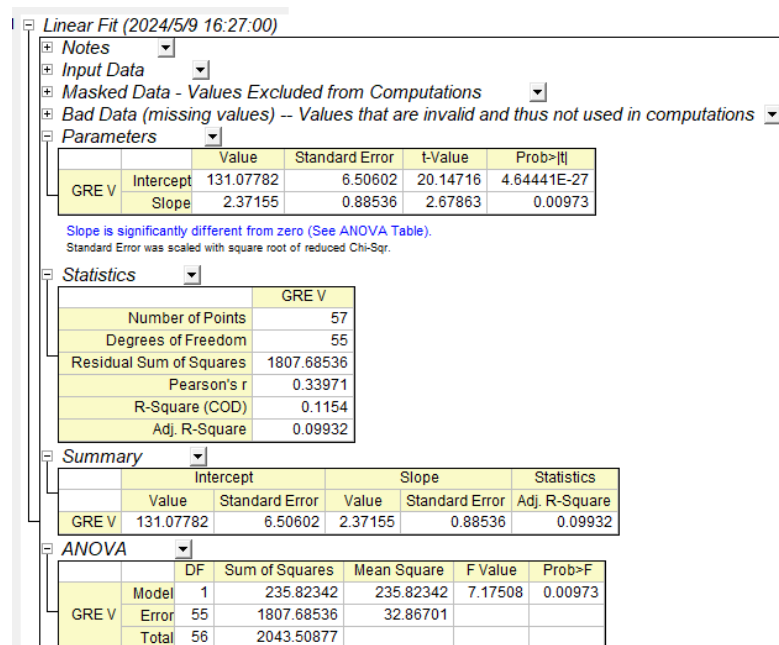
Figure 6. Regression analysis of IELTS reading scores and GRE verbal scores 图 6. 雅思阅读分数与 GRE 语文分数回归分析
