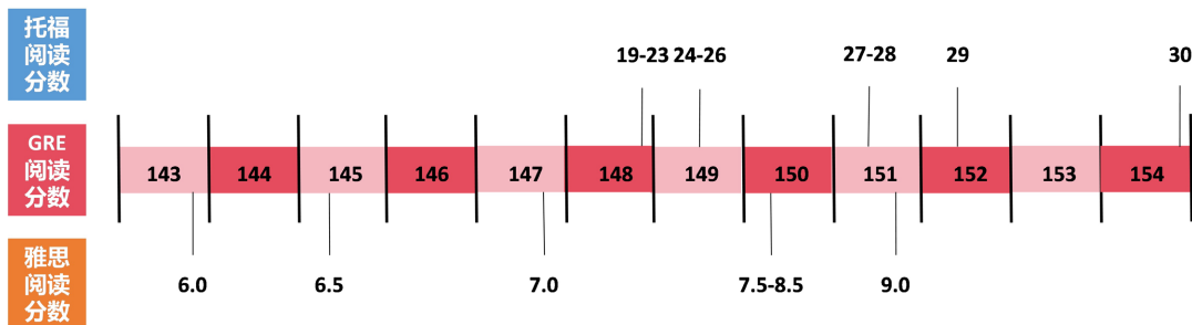
Figure 4. GRE verbal score corresponding to TOEFL/IELTS reading scores
