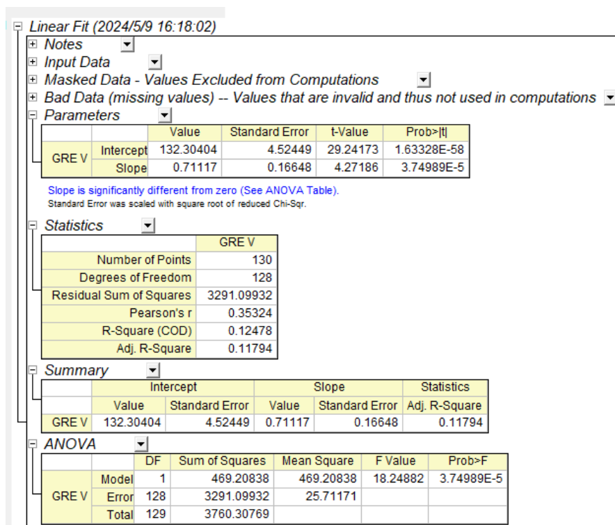
Figure 5. Regression analysis of TOEFL reading scores and GRE verbal scores
