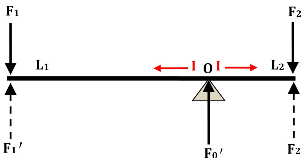
Figure 2. Schematic diagram of lever stress analysis
